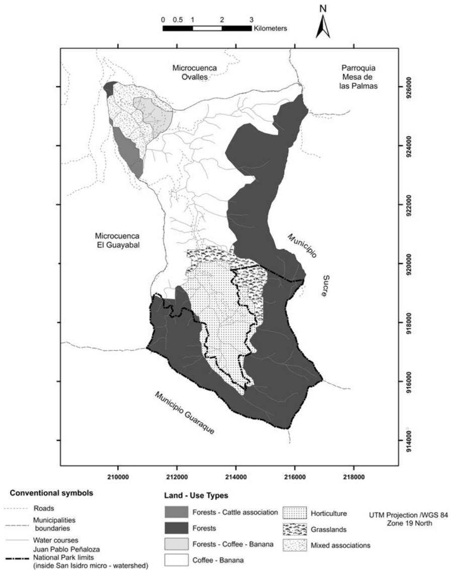
Fig. 2 Land-use map of the San Isidro micro-watershed in the Venezuelan Andes, Mérida state. Source Alciatiuri (2008)
